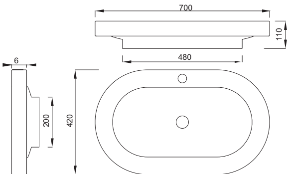
Lavello "ULAHOP 0" Basin "ULAHOP 0"
