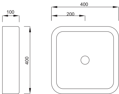
Lavello "LENS 40" Basin "LENS 40"
