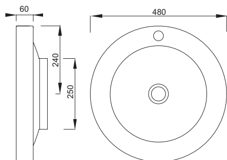
Lavello "ULAHOP R" Basin "ULAHOP R"
