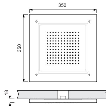
Soffione ad appoggio Shower head surface mounted
