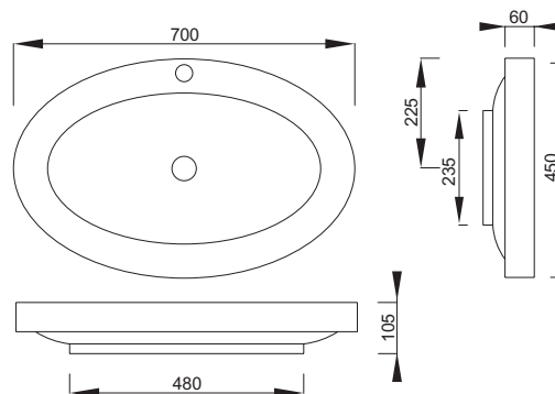
Lavello "ULAHOP E" Basin "ULAHOP E"
