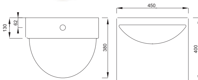
Lavello "WALL MINI" Basin "WALL MINI"
