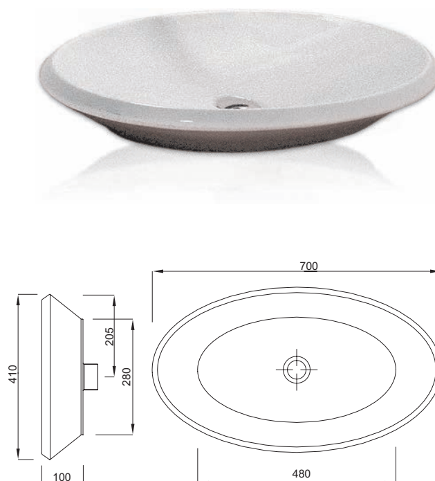
Lavello "OVAL" Basin "OVAL"
