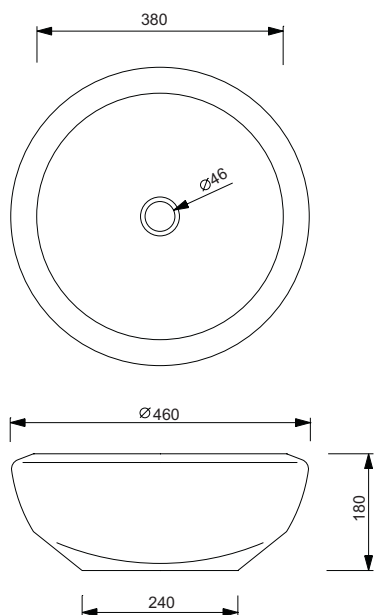
Lavello "BLEND 46" Basin "BLEND 46"
