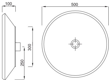
Lavello "PLAY" Basin "PLAY"
